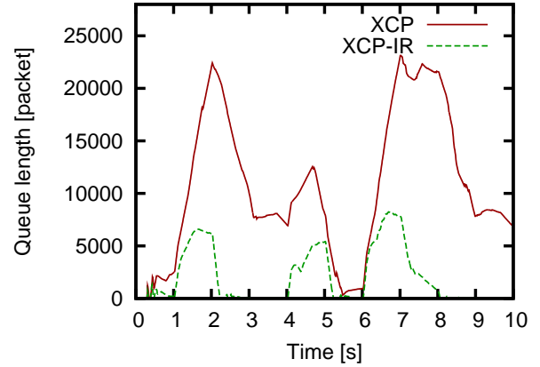
Fig. 12: Evolution of the queue length when suddenly changing the transfer rate of background UDP traffic
