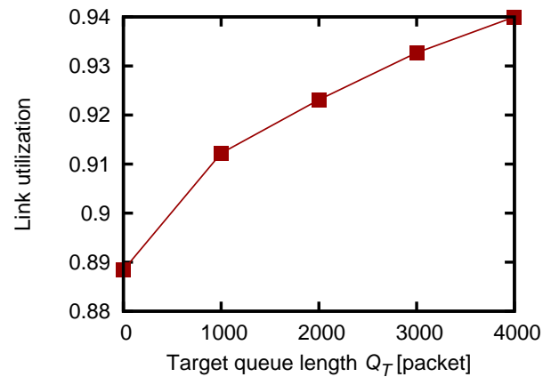
Fig. 6: Utilization of the bottleneck link for a different target value of the queue length Q_T (XCP corresponds to the case of Q_T = 0 )
