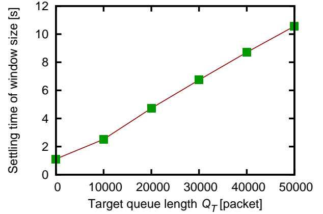
Fig. 8: Settling time of the window size when an XCP flow starts transfer from the initial state
