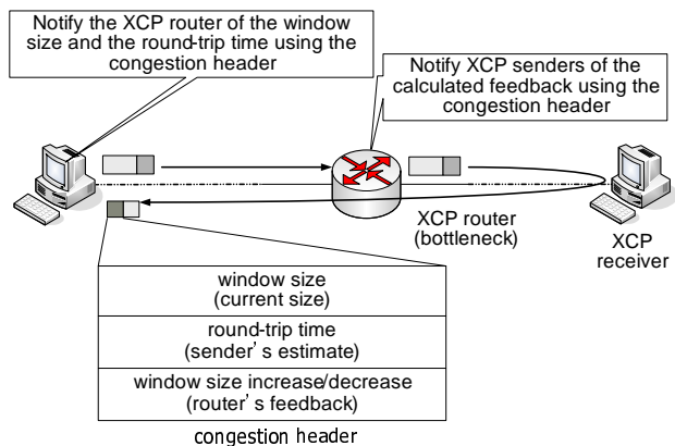
Fig. 1: Overview of XCP congestion control using congestion header
