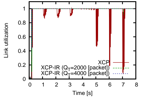
Fig. 9: Evolution of utilization of the bottleneck link for a different target value of the queue length Q_T
