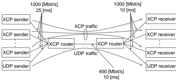
Fig. 4: Network topology used in simulation
