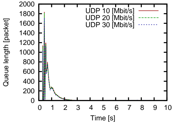
Fig. 10: Evolution of the queue length in XCP-IR when transmitting non-XCP traffic (UDP traffic)
