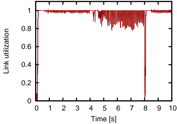
Fig. 2: Evolution of the utilization of the bottleneck link when changing the number of active XCP flows
