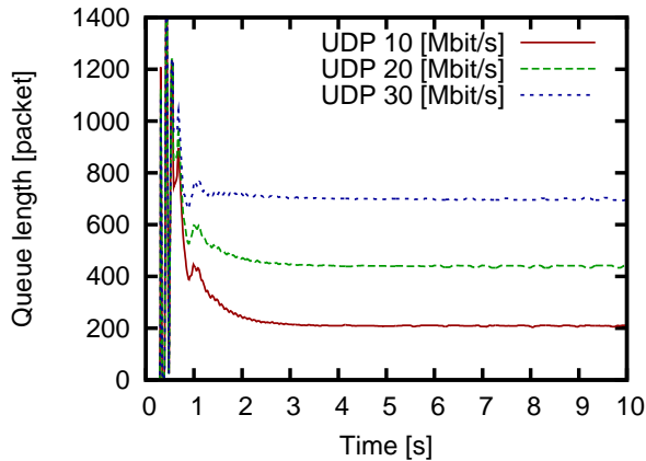
Fig. 3: Evolution of the queue length in XCP when transmitting non-XCP traffic (UDP traffic)
