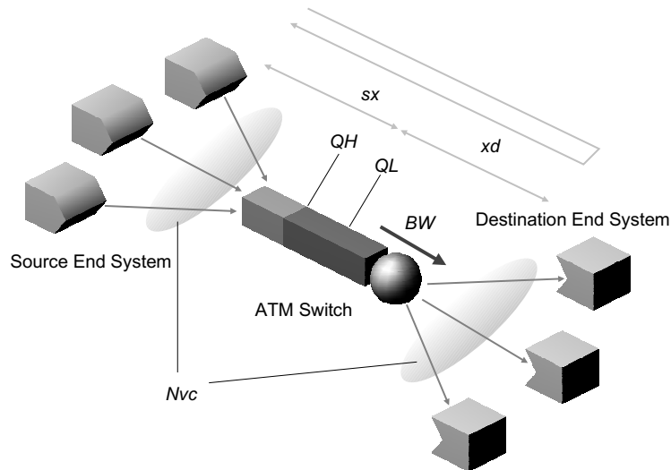
Figure 1: Analytic Model.
