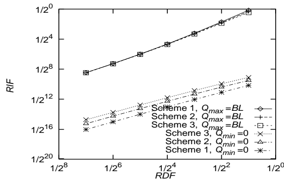
Figure 18: Analytic Results for Appropriate Parameters for \tau_{xx} = 0.01 .
