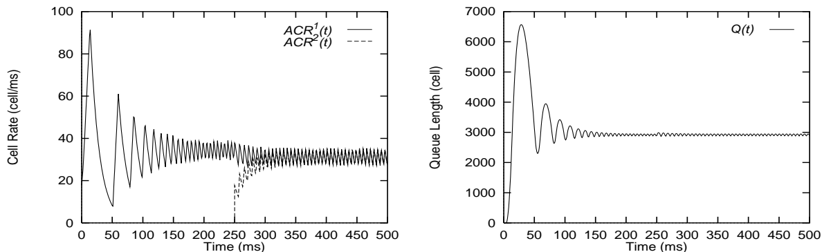
Figure 5: Effect of Propagation Delay for \tau_1 = 0.02 ms and \tau_2 = 0.02 ms.
