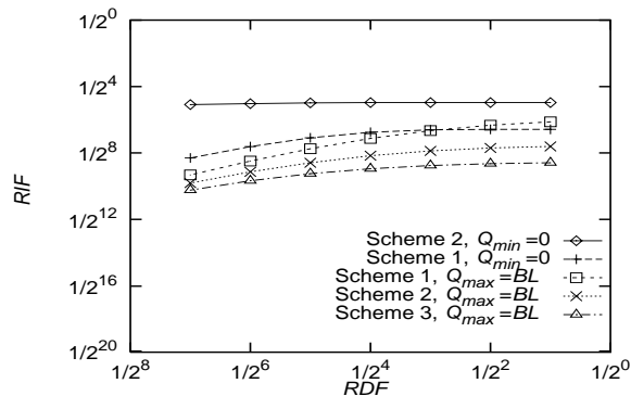
Figure 20: Analytic Results for Appropriate Parameters for \tau_{xx} = 1.00 .
