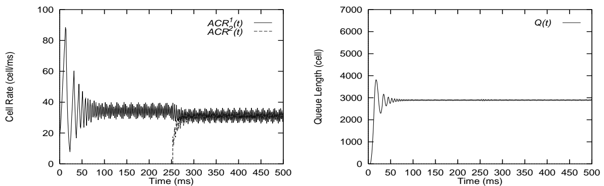
Figure 8: Effect of Control Parameters for RIF = 1/64 and RDF = 1/4 .
