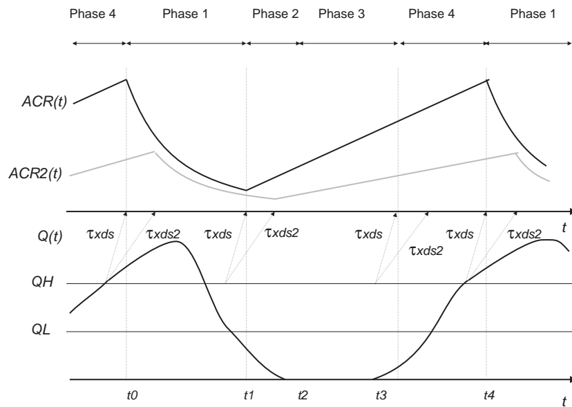
Figure 4: Pictorial View of ACR^n(t) and Q(t) .
