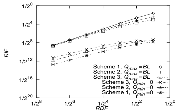
Figure 19: Analytic Results for Appropriate Parameters for \tau_{xx} = 0.10 .
