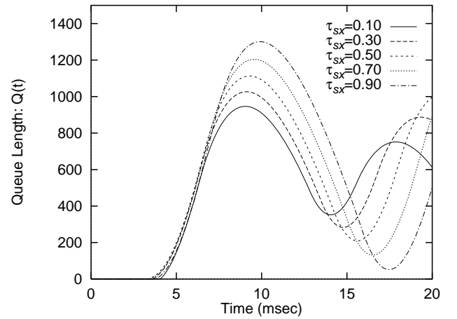
Fig. 6: Effect of Switch Location on Q(t) in BES Switch ( N_{VC} = 10 ).
